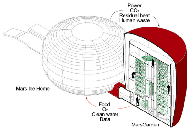
Fig. 1. Axonometry of MarsGarden coupled with the Mars Ice Home.
