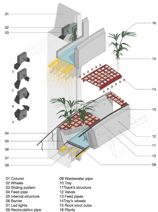
Fig. 6. Detailed section of the helical hydroponic system.
