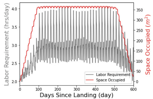
Fig. 4. Dynamics of the required human labor (hours per day) and required growing surface area (square meters) over a 600 Earth day mission on Mars for a crew of four astronauts.
