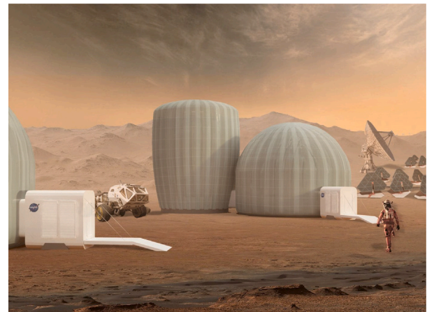
Fig. 2. Rendered image of MarsGarden coupled with the Mars Ice Home.
