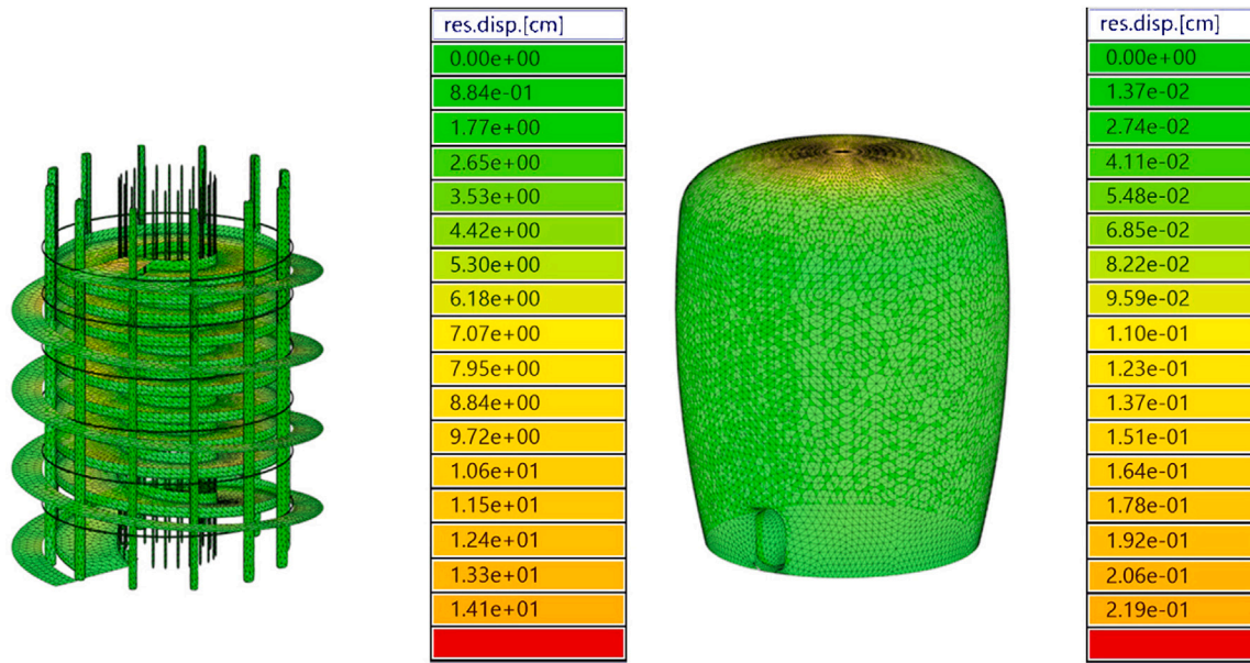
Fig. 8. Results of the FEM simulation of the module.
