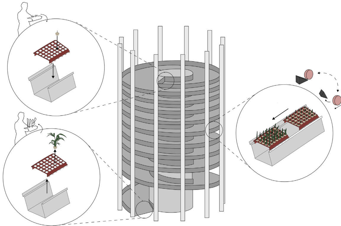
Fig. 7. Trays movement detail: astronauts place the trays on the spiral track with fresh seedlings (top left), trays passively shift down the track over the course of the crop's lifetime (middle right), and astronauts lift the trays out when plants are mature and reach the bottom of the spiral (bottom left).
